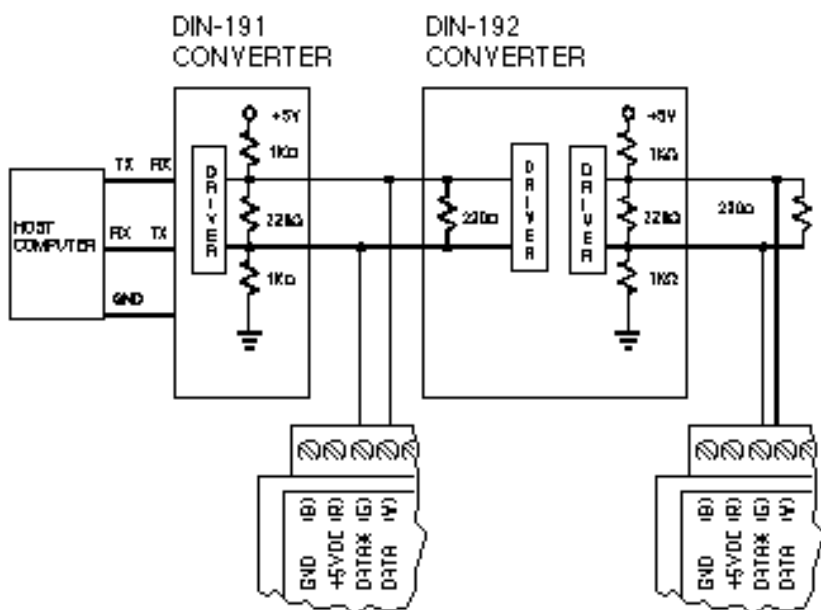
Figure 2. RS-485 biasing & termination resistors.
