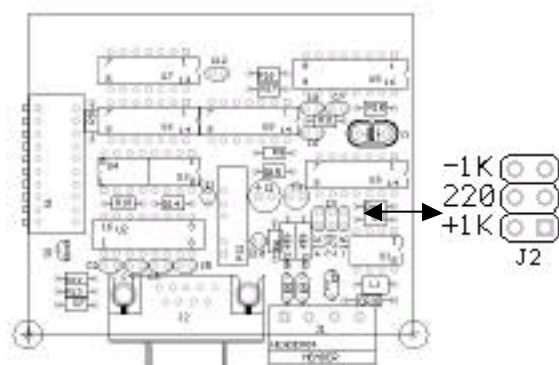
Figure 3. DIN-191 jumper locations.
