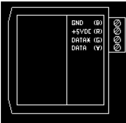
Figure 1A Connections for DIN-191.
