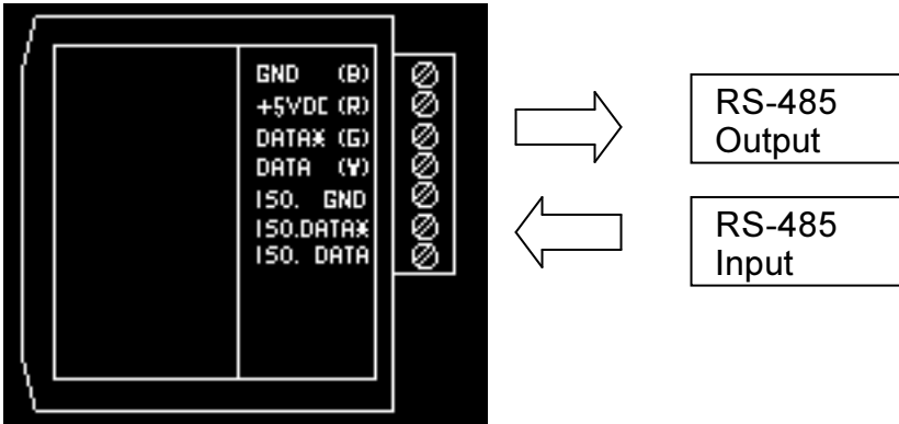
Figure 1B Connections for DIN-192.
